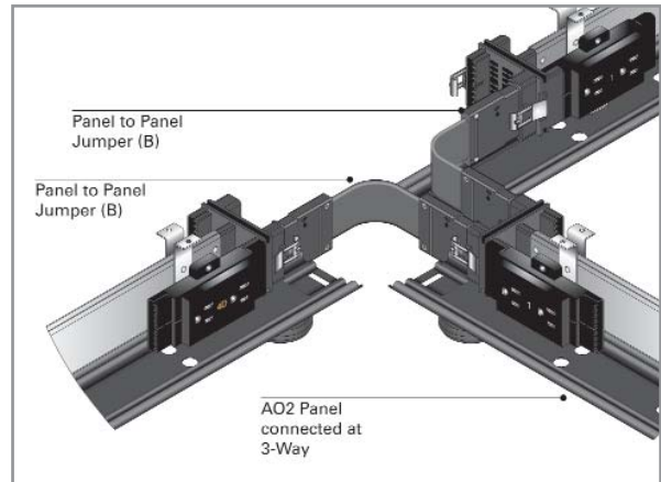
AO2 electrical, 8-wire, 4-circuit 3-way 90-degree connector. Used to connect 3 adjacent powered panels of any width at 90-degrees.
