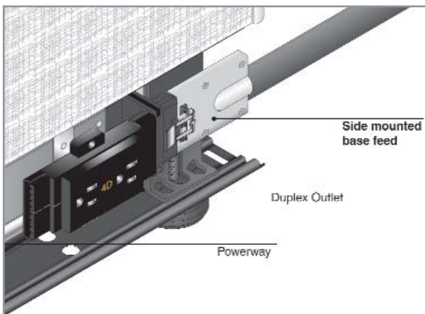
AO2 electrical 8-wire, 4-circuit side mounted base feed. Used to connect building power supply to the base of the wall or floor monument.
